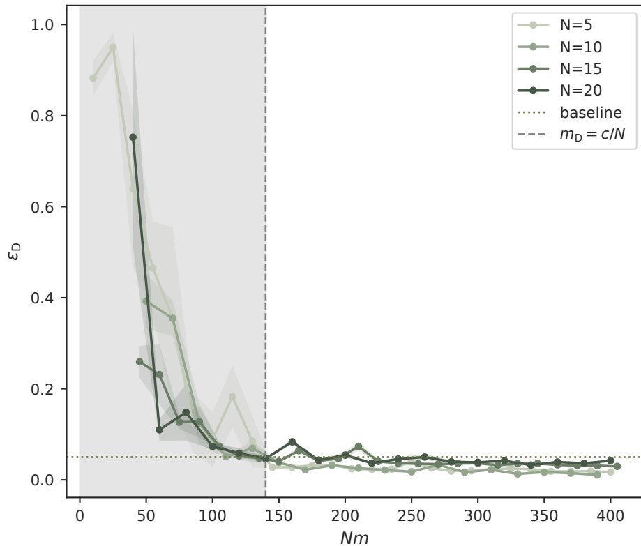
Lorenz knstruc (best over epochs): max component error
